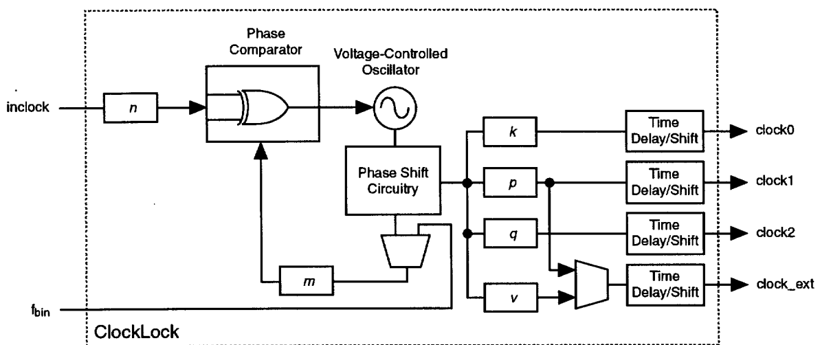
Figure 31. Mercury General-Purpose PLL
