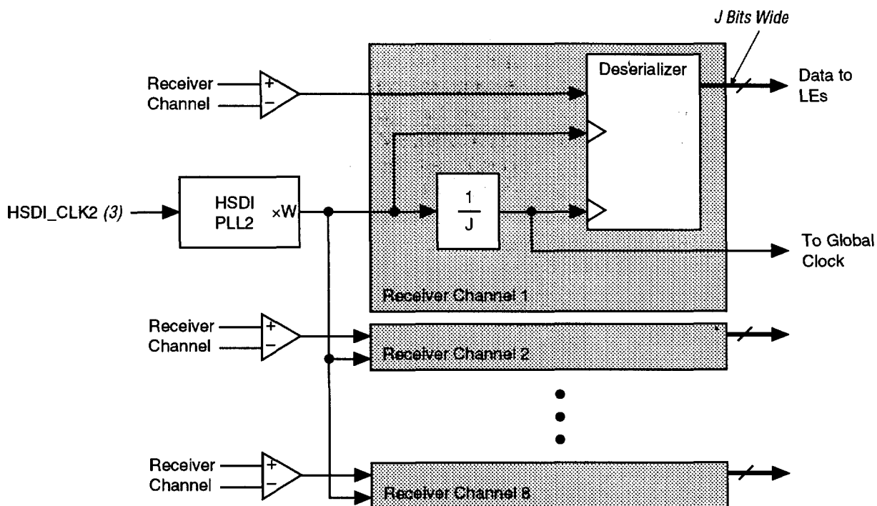
Figure 2. Receiver Diagram for Source Synchronous Mode Notes (1), (2)
