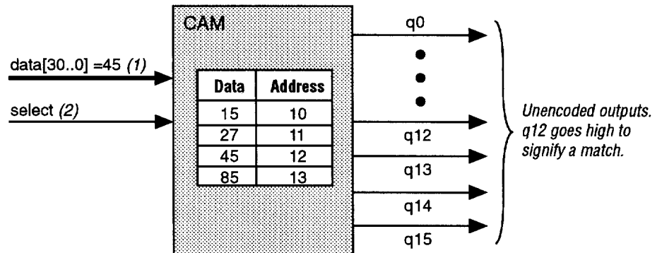
Figure 24. Unencoded CAM Address Outputs
