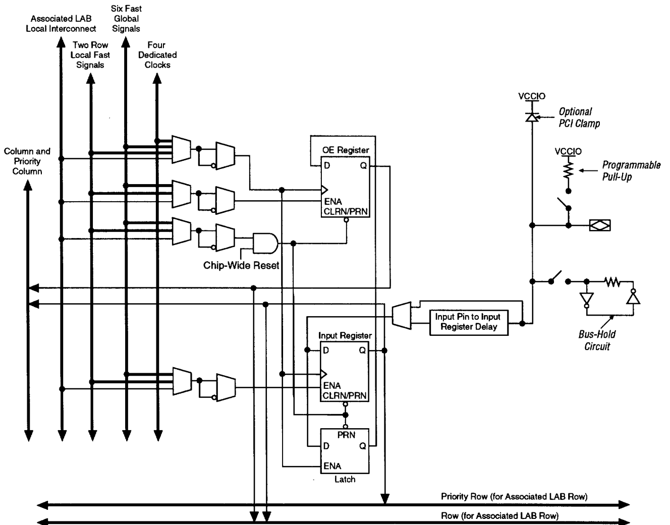
Figure 27. IOE Configured for DDR Input
