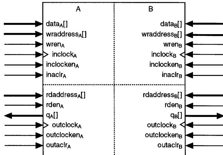
Figure 17. ESB Quad-Port Block Diagram
