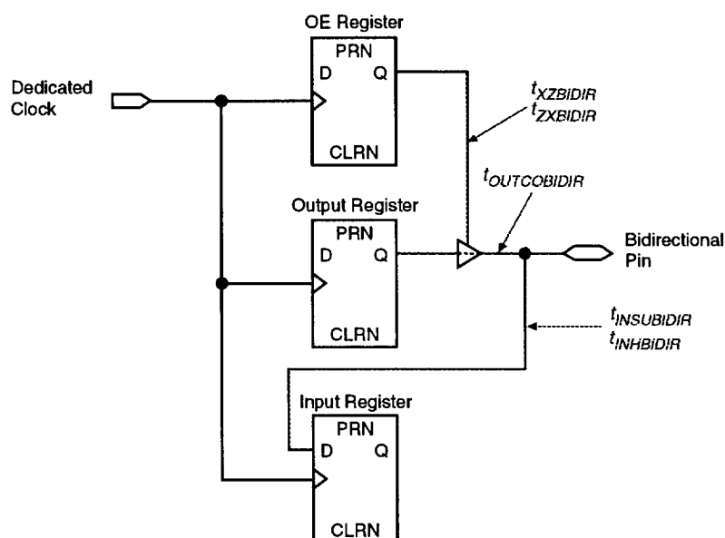
Figure 34. Synchronous Bidirectional Pin External Timing Model
