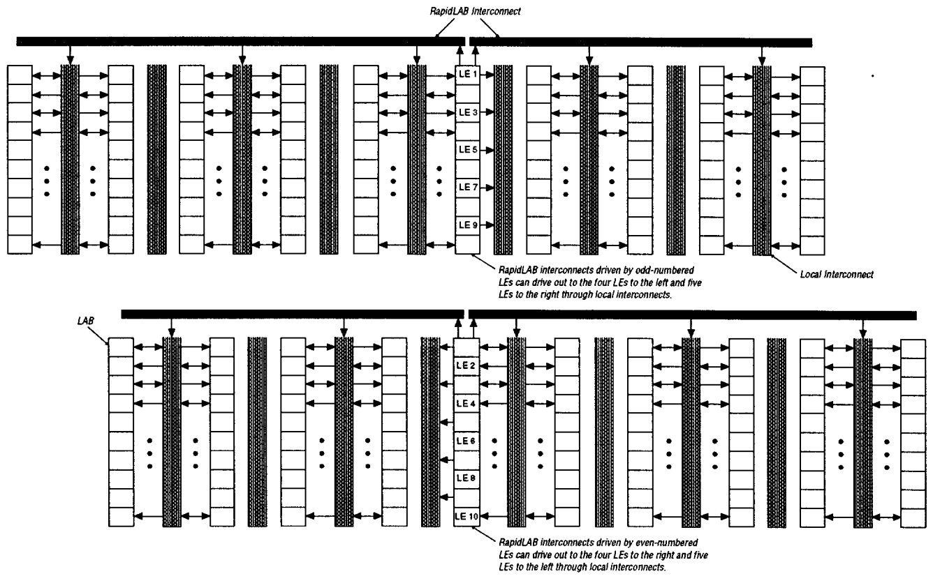
Figure 14. RapidLAB Interconnect Connections
