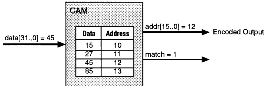
Figure 23. Encoded CAM Address Outputs
