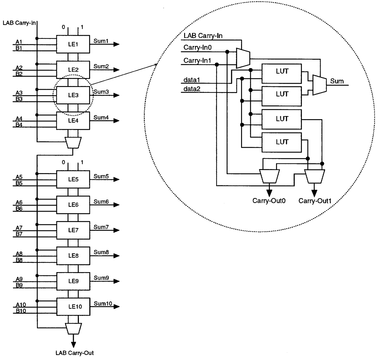
Figure 10. CSLA Details
