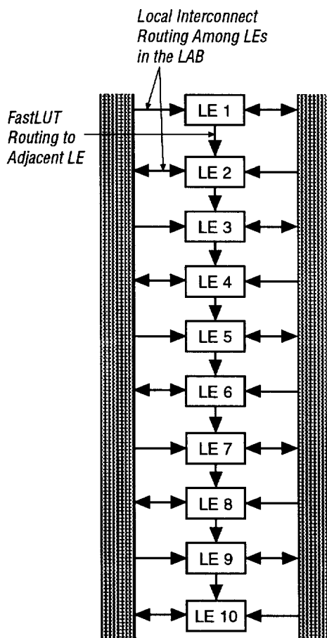
Figure 16. FastLUT Interconnect
