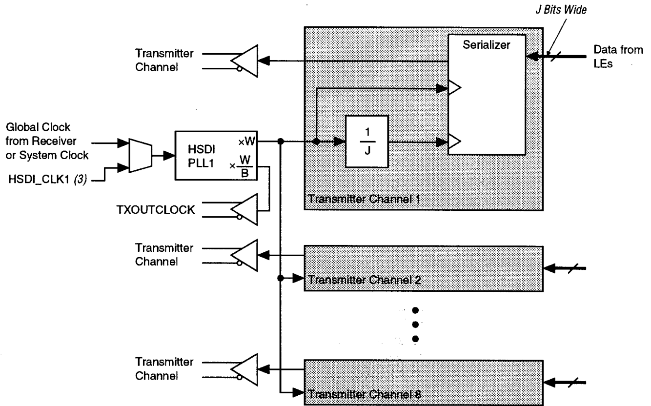
Figure 3. Transmitter Diagram for Source Synchronous Mode Notes (1), (2)
