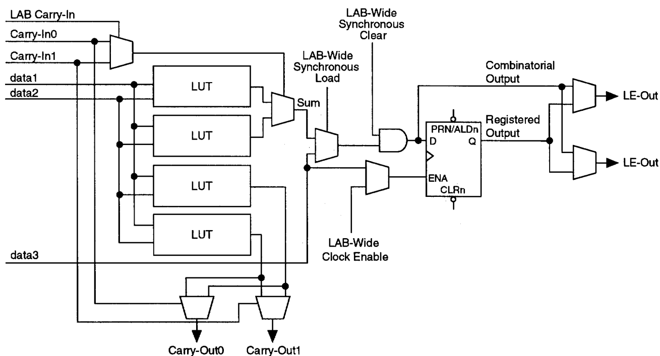
Figure 9. Arithmetic Mode LE
