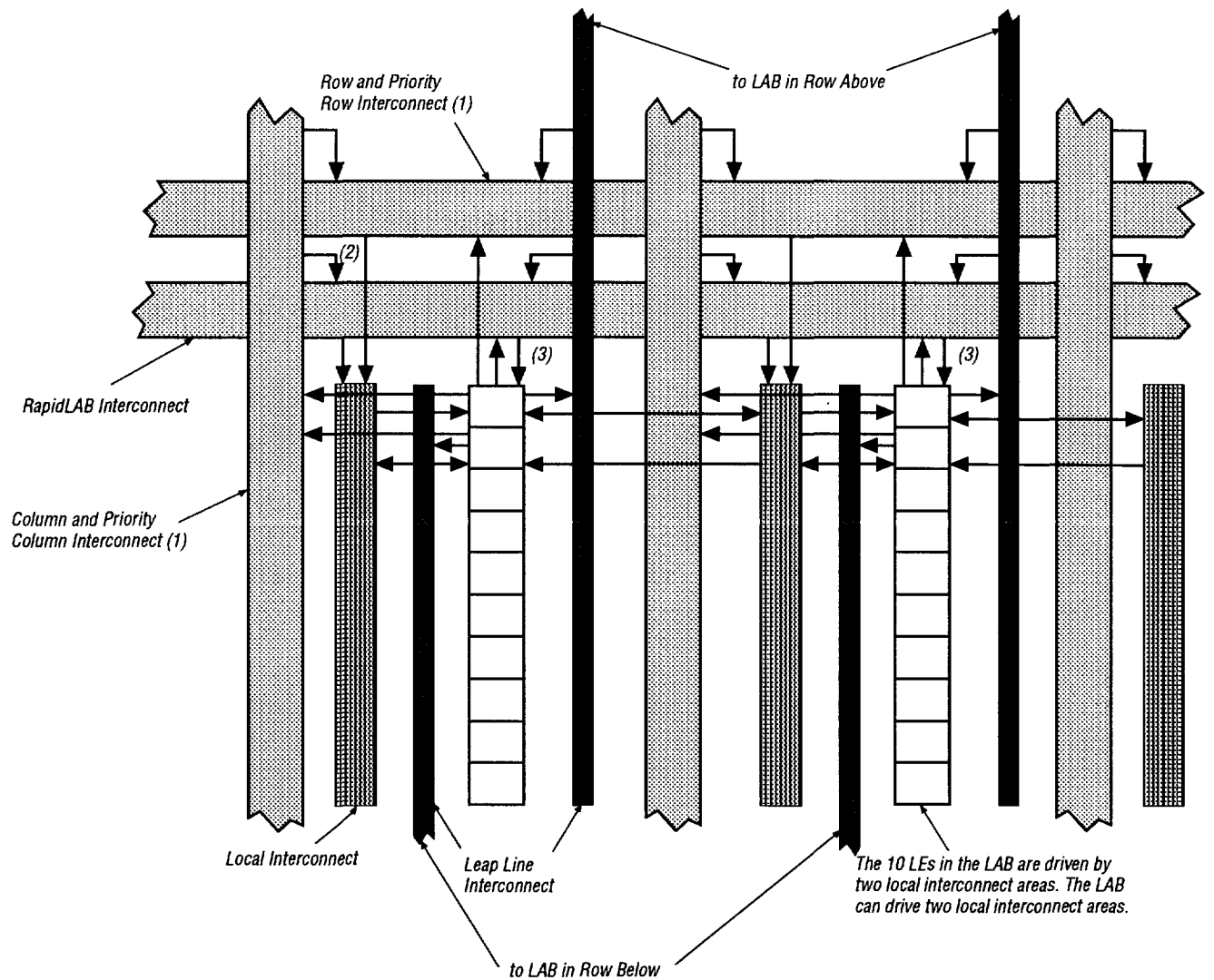
Figure 5. Mercury LAB Structure
