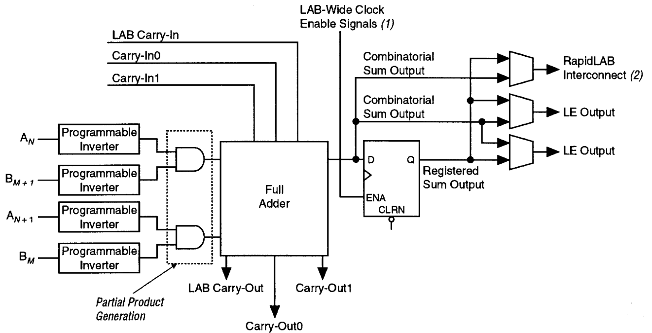
Figure 11. Multiplier Mode LE
