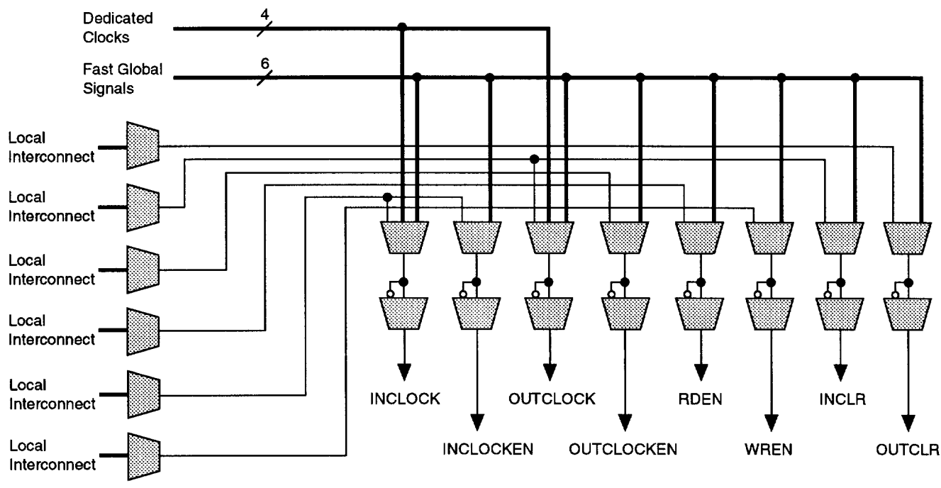
Figure 25. ESB Control Signal Generation
