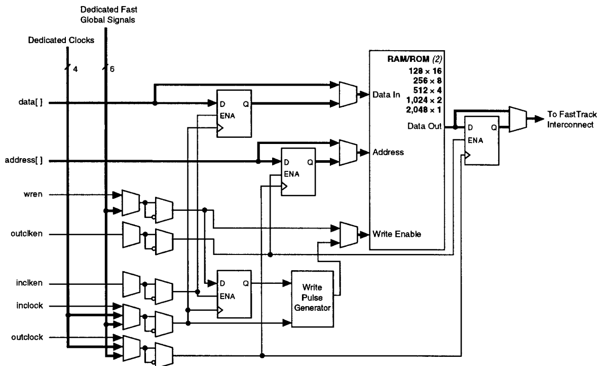
Figure 21. ESB in Single-Port Mode Note (1)
