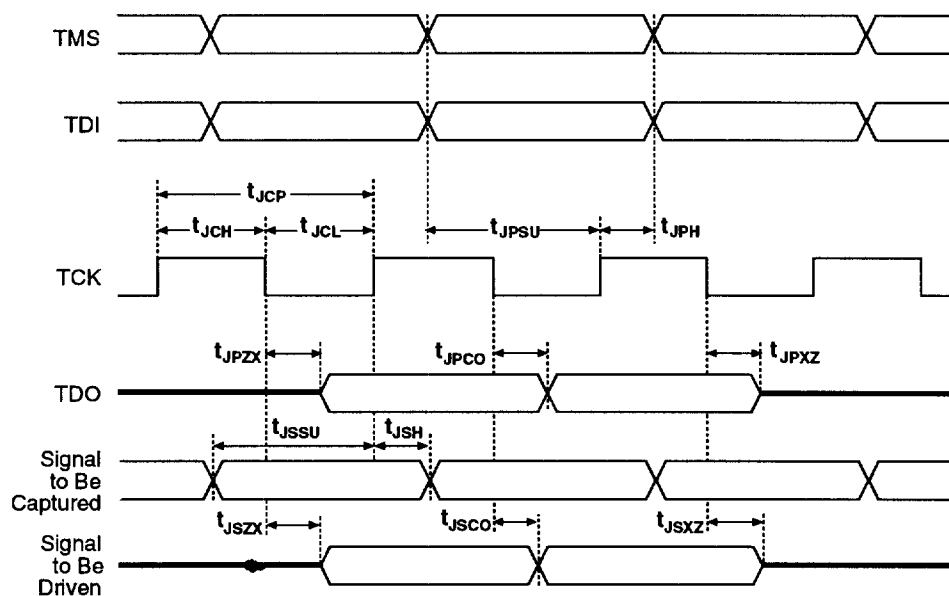
Figure 32. Mercury JTAG Waveforms
