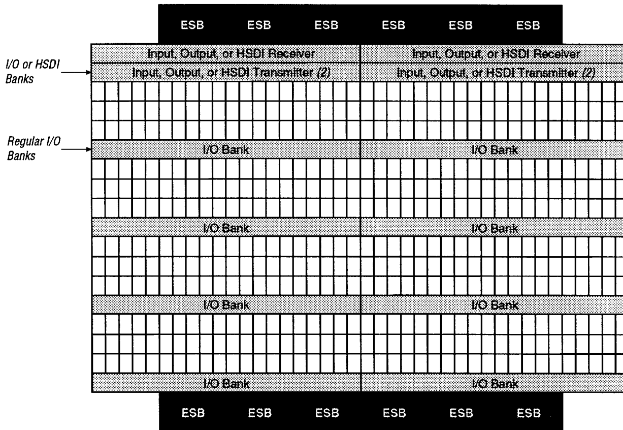
Figure 30. I/O Bank Layout
