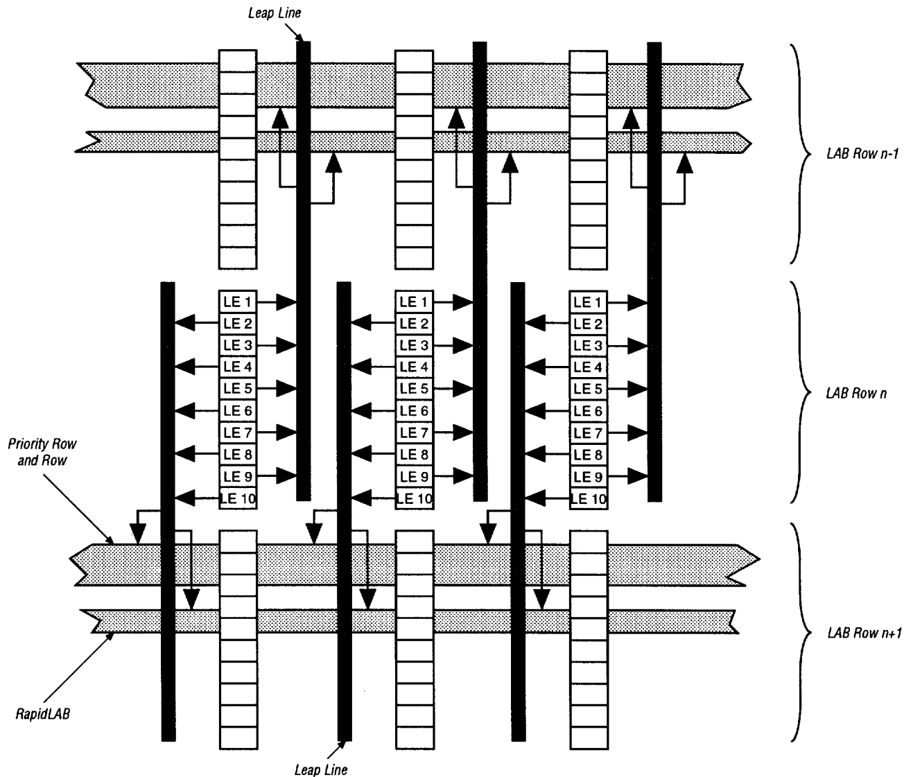
Figure 15. Leap Line Interconnect
