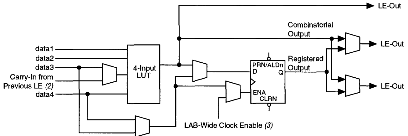
Figure 8. Normal-Mode LE Note (1)
